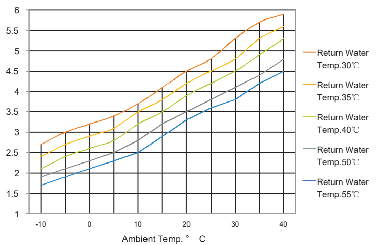
COP Curves
